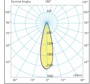
30° Lens
