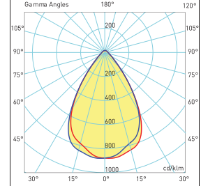
90° Lens
