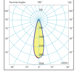
30° Lens
