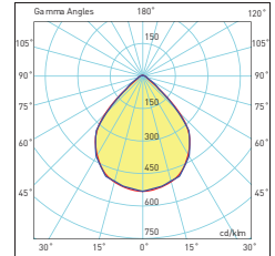
90° Lens
