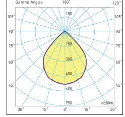
60° Lens
