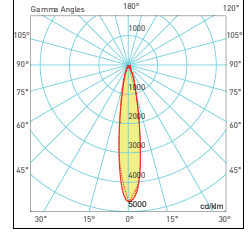
10° Lens
