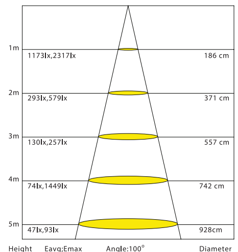
Conic Diagram - 5612 6161
